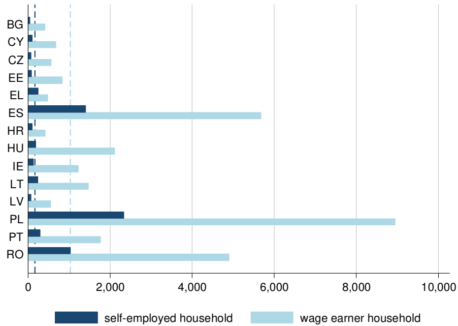
Figure A.1. Number of self-employed and wage earner households in the estimation sample
