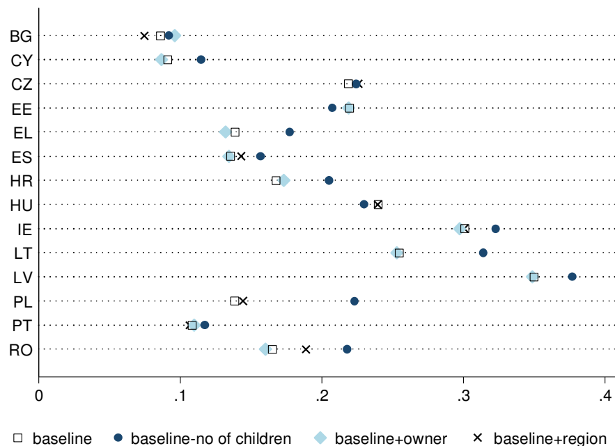
Figure 2. Estimates of the simple share of unreported income with alternative covariates
