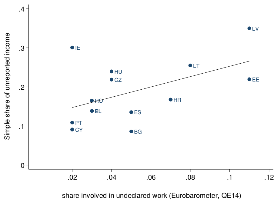
Figure 6. Estimates of the simple share of unreported income and the share of undeclared work
