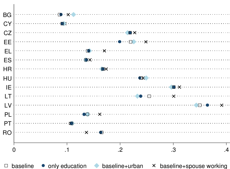
Figure 3. Estimates of the simple share of unreported income with alternative instruments
