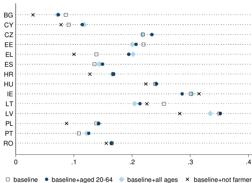
Figure 4. Estimates of the simple share of unreported income with alternative samples
