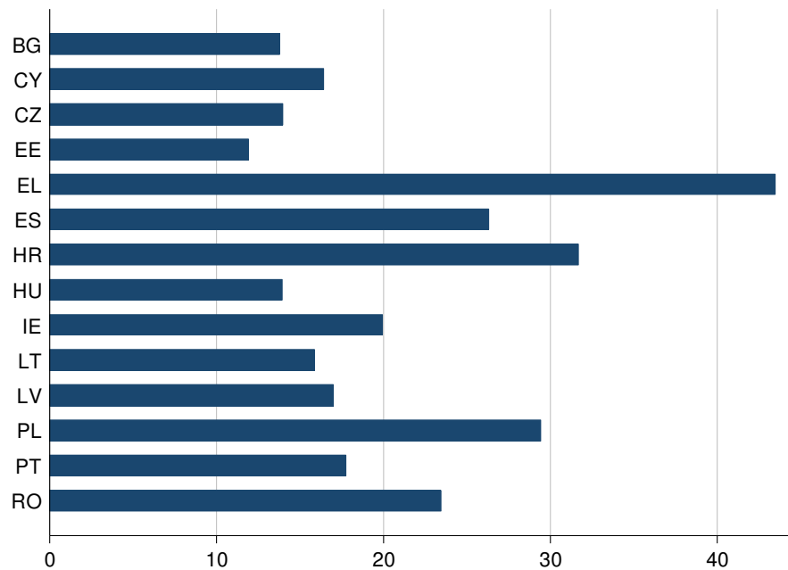
Figure A.2. Percentage of self-employed households in the estimation sample
