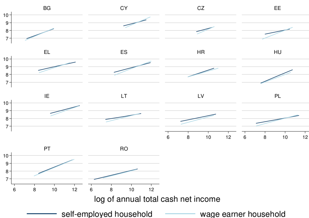
Figure 1. Linear Engel curves for household food consumption
