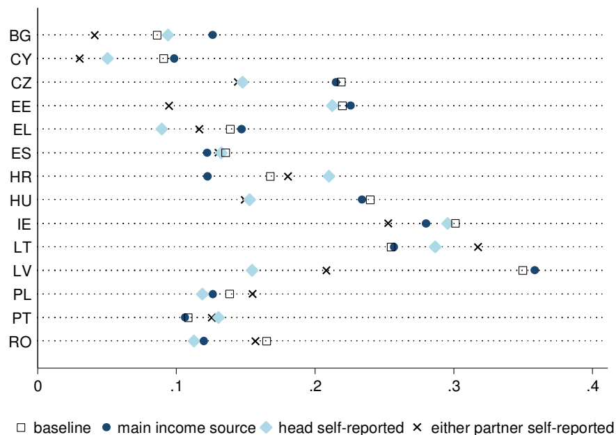
Figure 5. Estimates of the simple share of unreported income with alternative definitions of self-employed households
