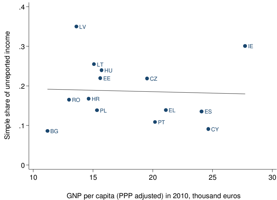
Figure 7. Estimates of the simple share of unreported income and GNP per capita (PPP)
